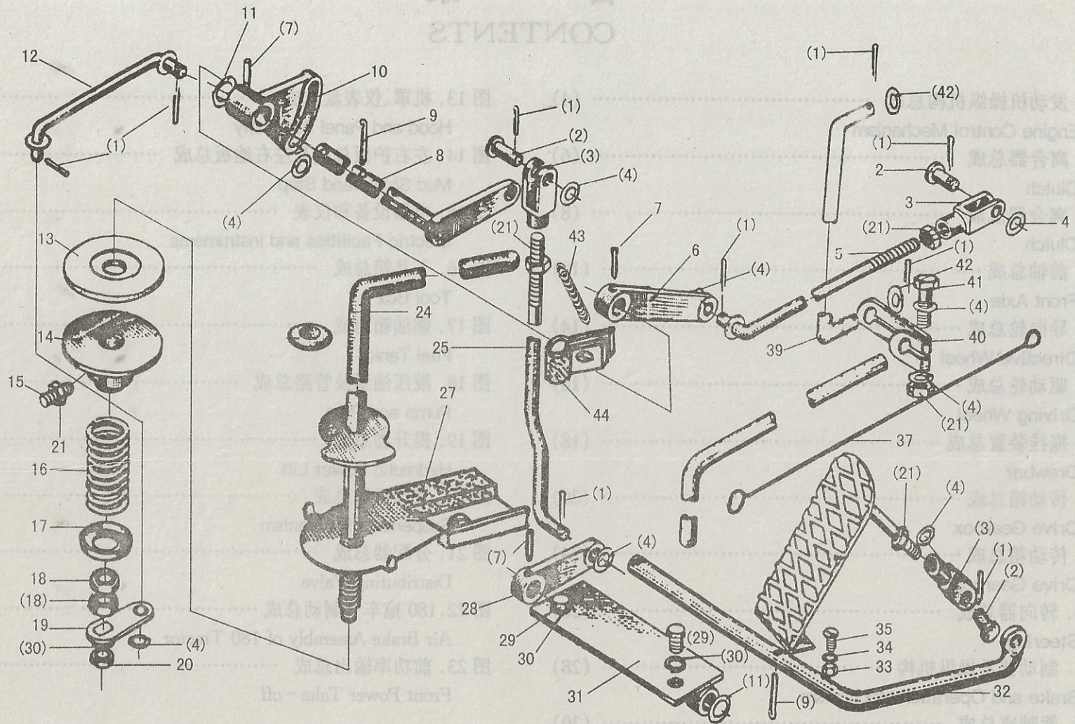
Fig.1 Engine Control mechanism
