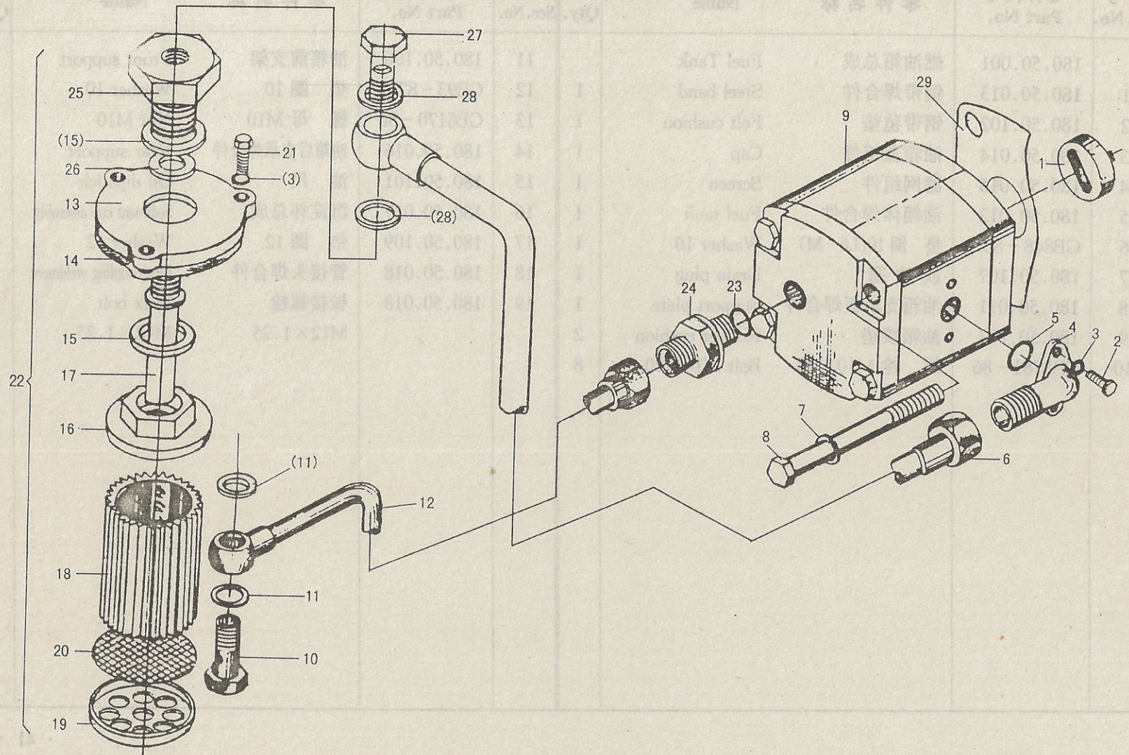
Fig.18 Pump and pipe
