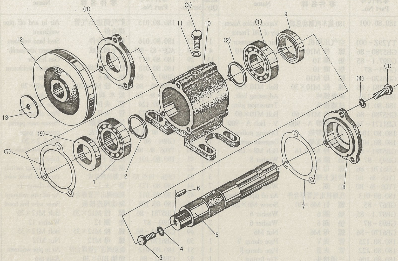
Fig.23 Front Power Take - off
