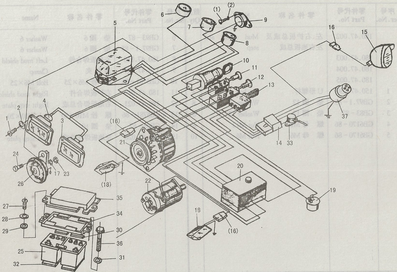
图 15. 电器设备和仪表 Fig.15 Electric Facilities and Instruments
