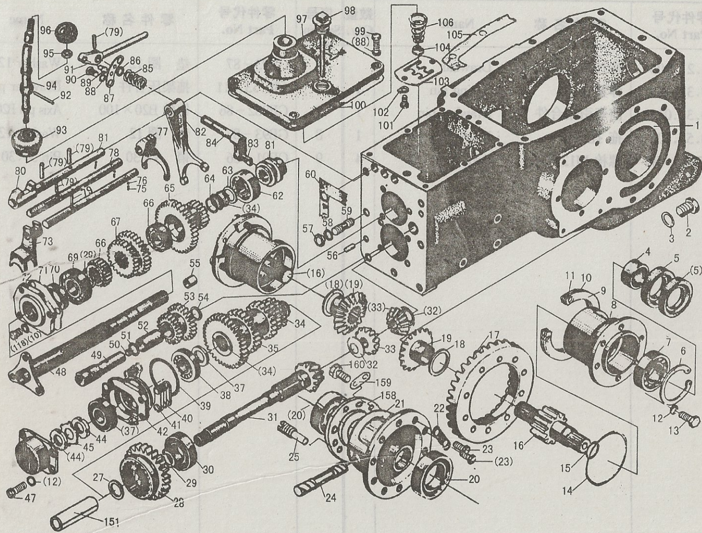
Fig.8 Drive Gearbox
