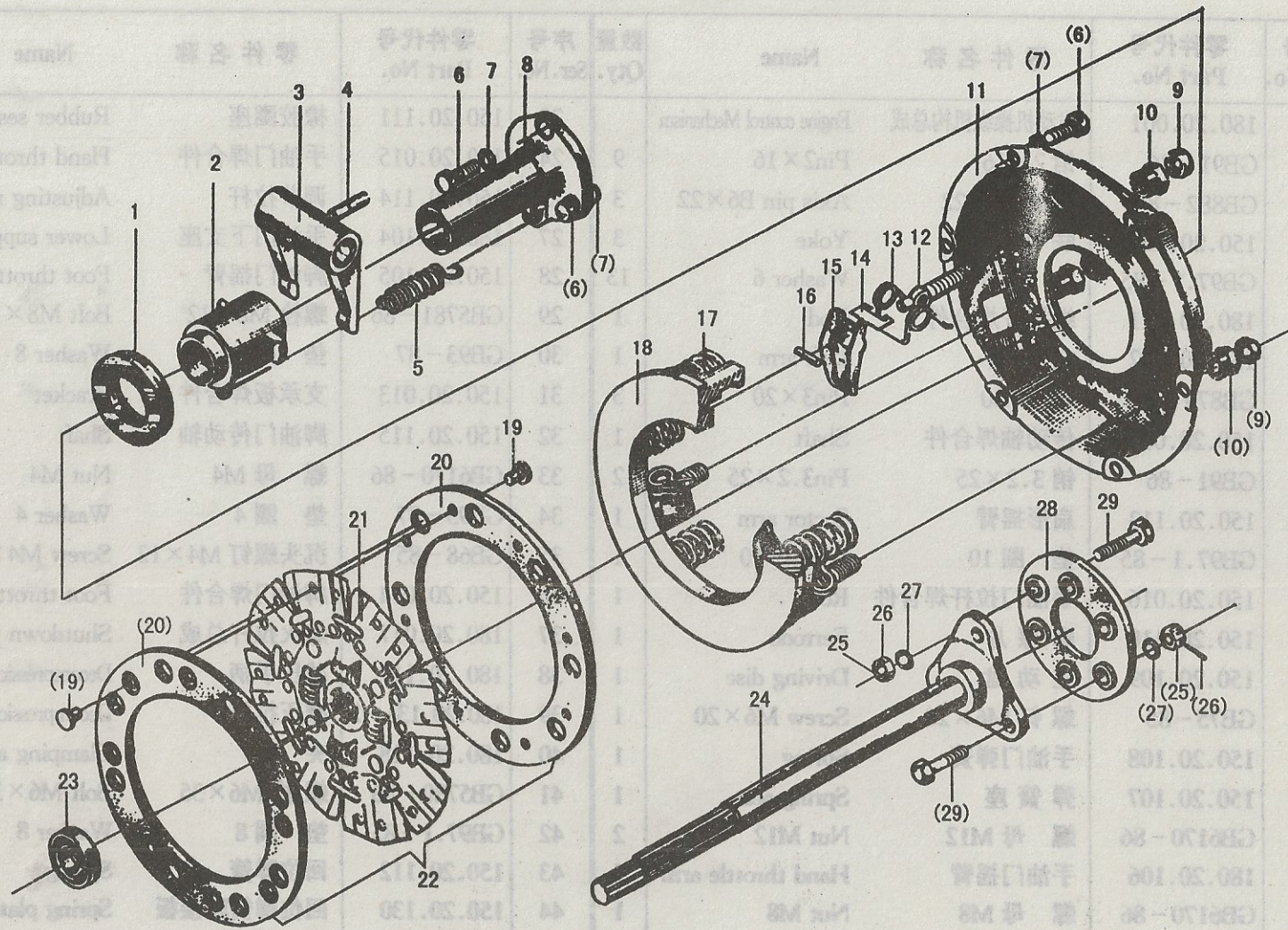
Fig.2 Clutch
